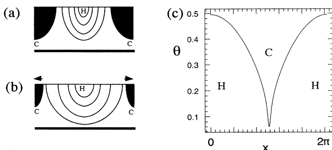
FIG. 7. Illustration of the nonlinear redistribution of temperature in high-Prandtl-number Bénard-Marangoni convection: Sketch of the temperature isolines of a pair of rolls in the (a) weakly nonlinear and in (b) strongly nonlinear regime. Surface temperature field (c) of a deformed roll as obtained from direct numerical simulation of the infinite-Prandtl-number equations for Ma=2000 (aspect ratios l_x = \pi, l_y = 1 , spatial resolution 512 \times 32 \times 128 , Bi=0 ). H and C denote cold and hot regions.
